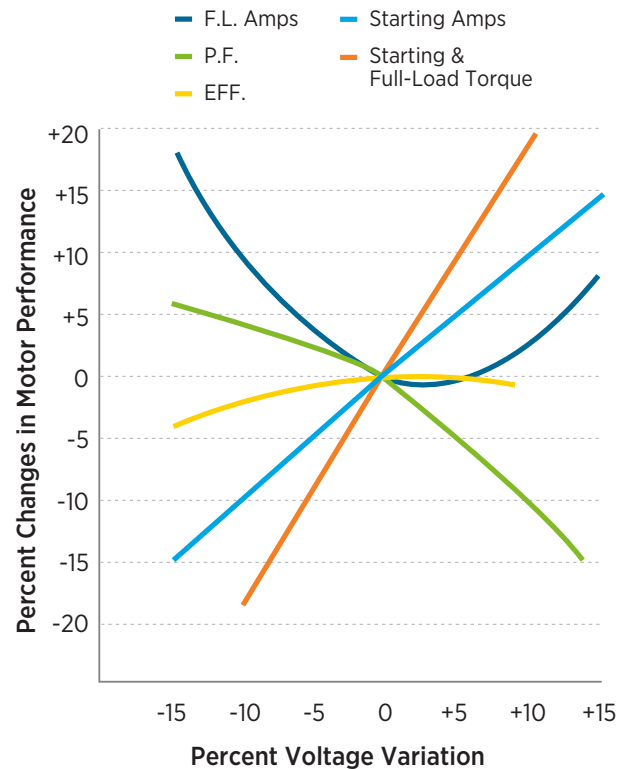
Figure 5-1. Voltage variation effect on standard efficiency motor performance
