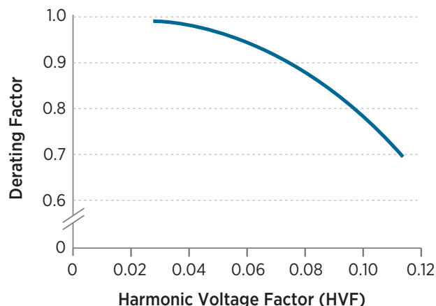
Figure 9-2. Harmonic voltage derating curve
