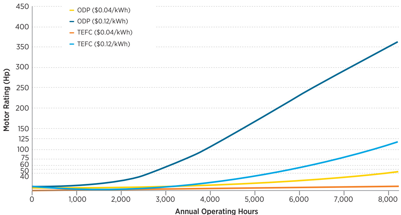
Figure 4-2. Horsepower breakpoint for replacing a failed motor with a premium efficiency motor
