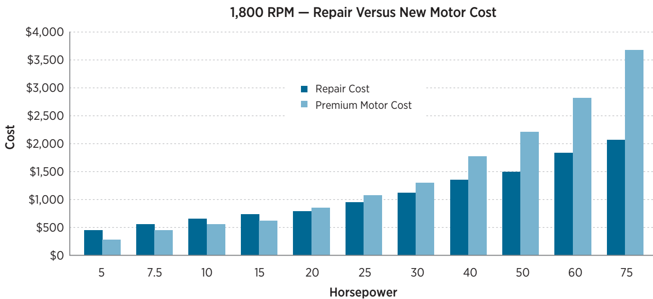
Figure 4-1. Motor repair (bearing replacement plus rewinding) and new premium efficiency motor costs (for 1,800 RPM TEFC motors, 2011 prices)
