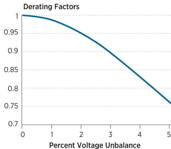
Figure 5-2. Motor derating due to voltage unbalance
