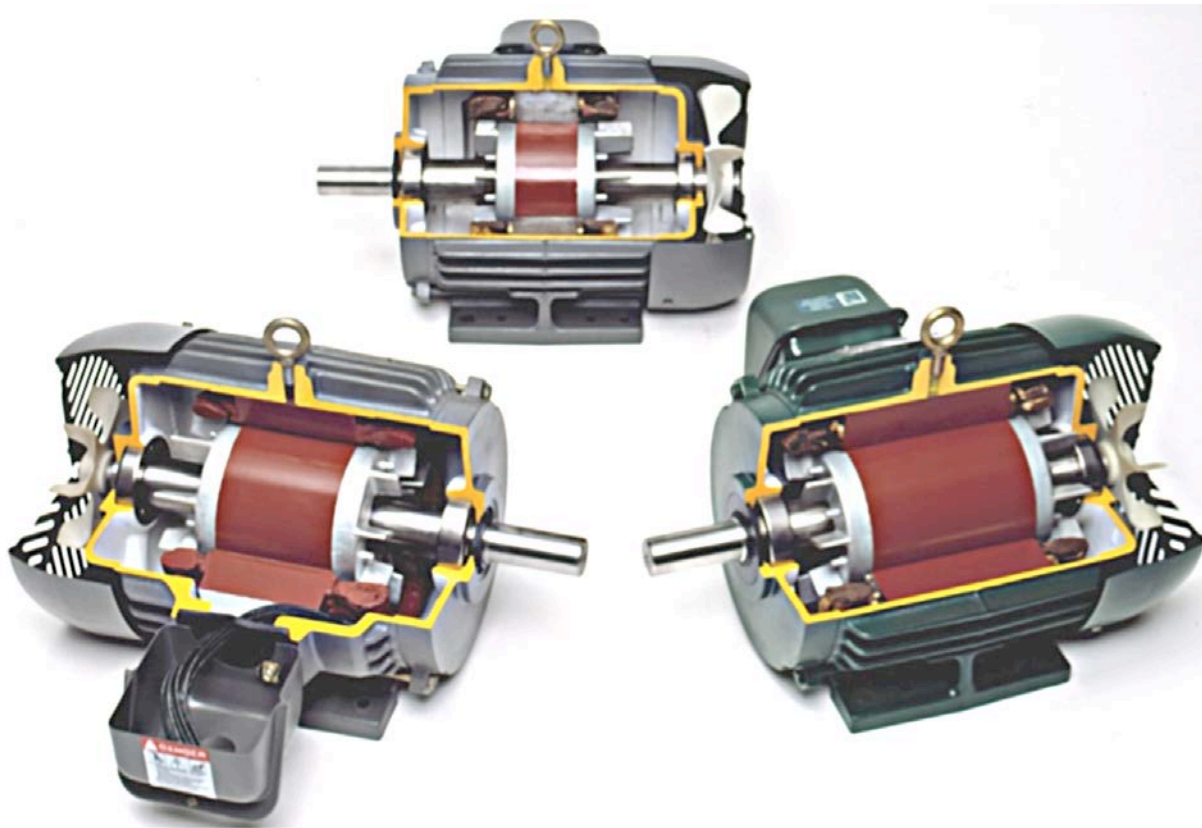
Figure 2-5. Cut-away of standard, energy-efficient, and premium efficiency motors. Photo from Toshiba International Corporation
